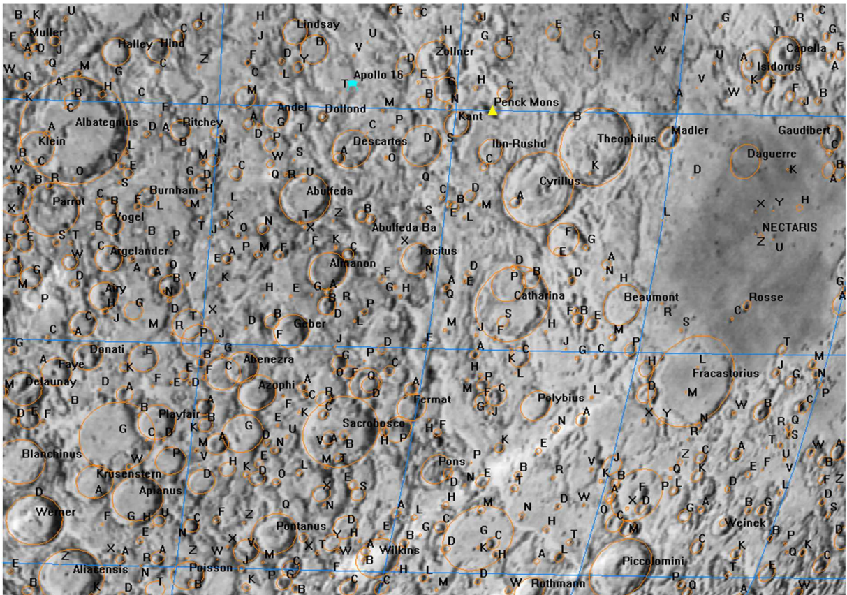
14. Catharina
