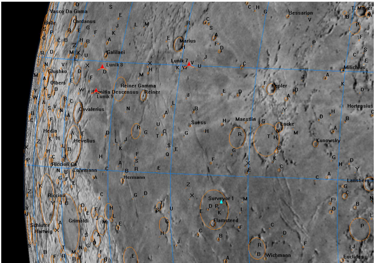
8. Kepler
