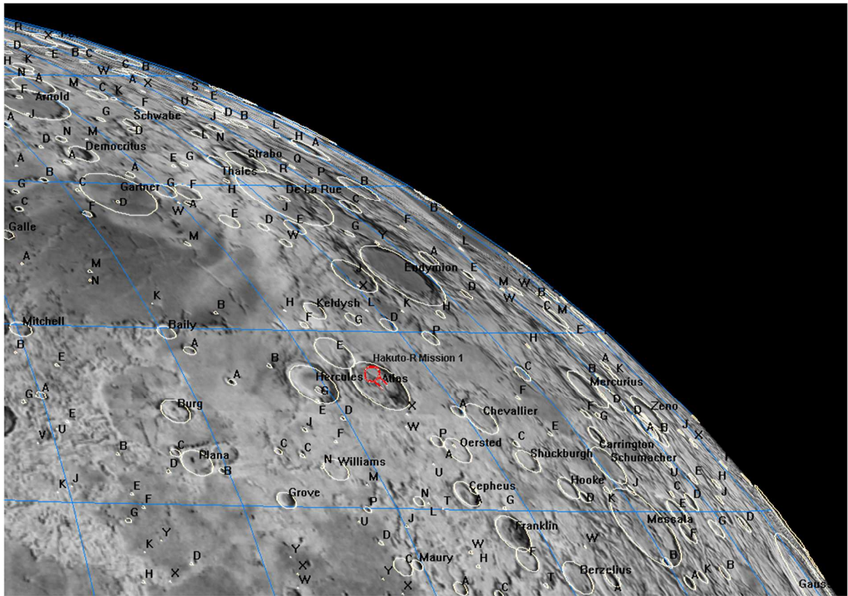
3. Endymion
